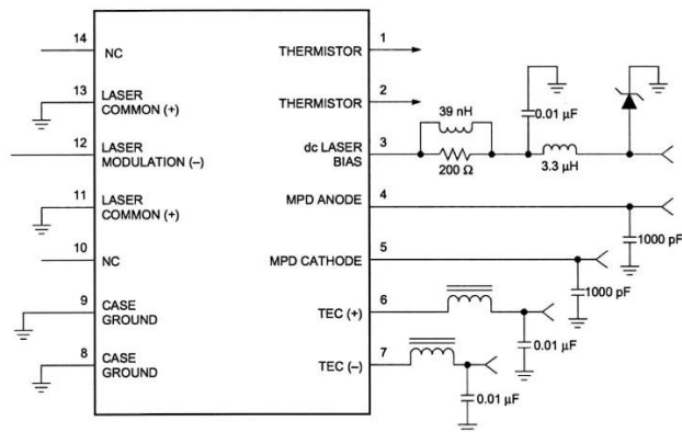
Figure 2. 1764 Circuit Schematic
